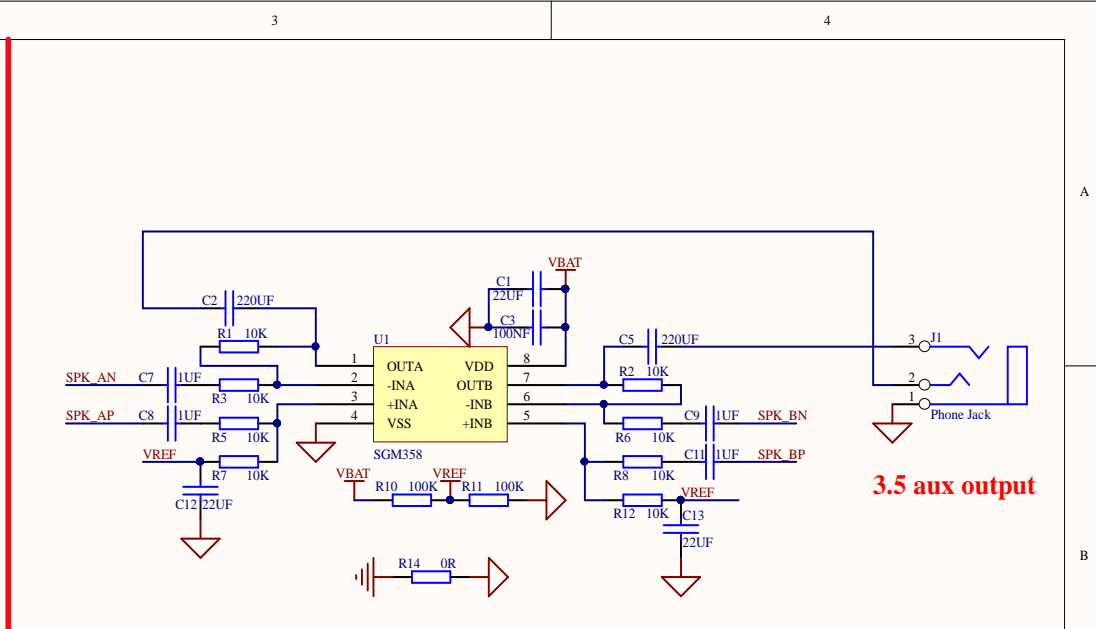
Differential to single-ended analog audio output
