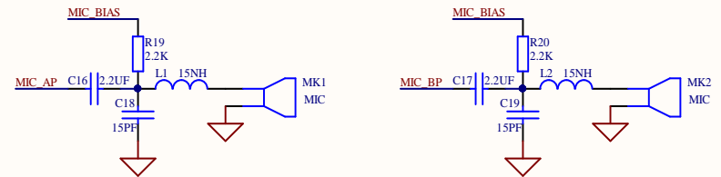
microphone input
