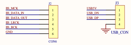
I2S Digital audio output
