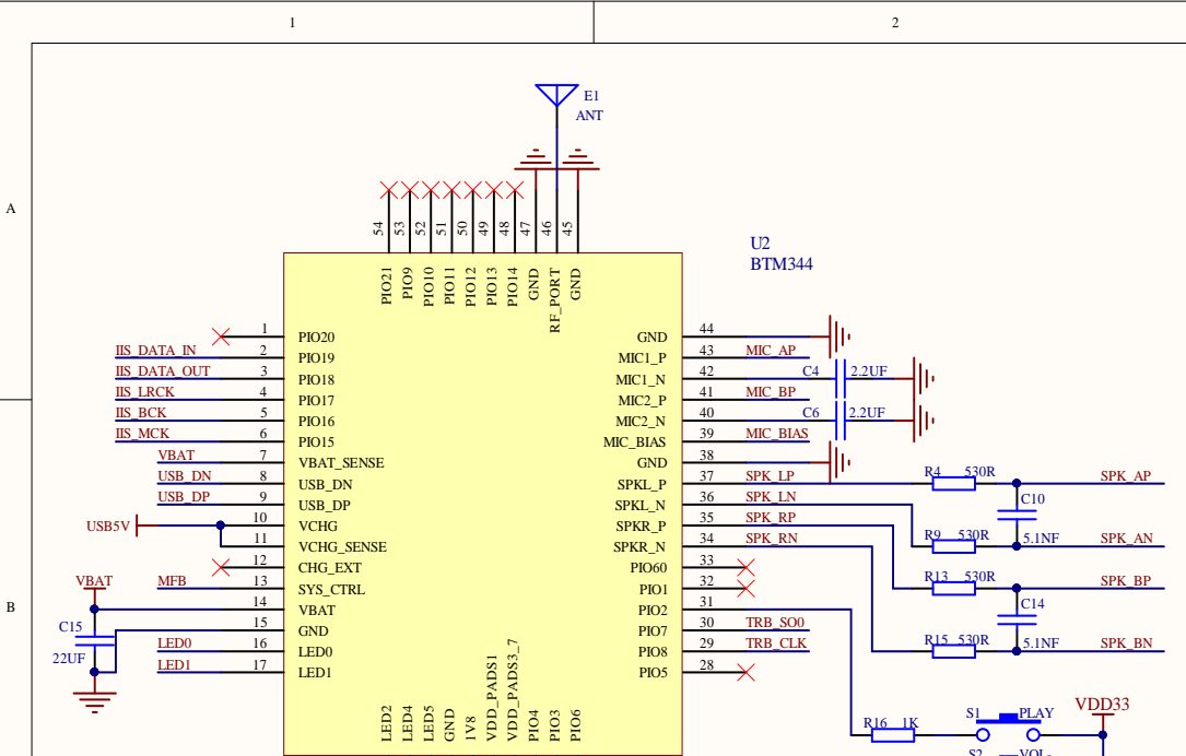
Differential to single-ended analog audio output
