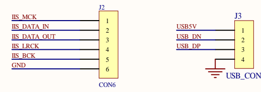
I2S Digital audio output
