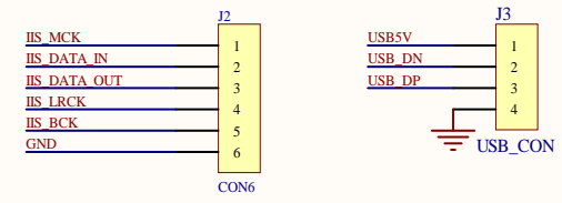
I2S Digital audio output
